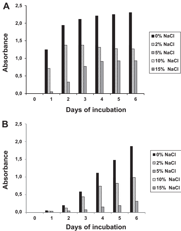
Fig. 3. Growth curves of Pseudomonas fluorescens S12N in the presence of several salt concentrations at 25 °C (A) and 5 °C (B). Absorbance was measured at 595 nm every 24 h.
