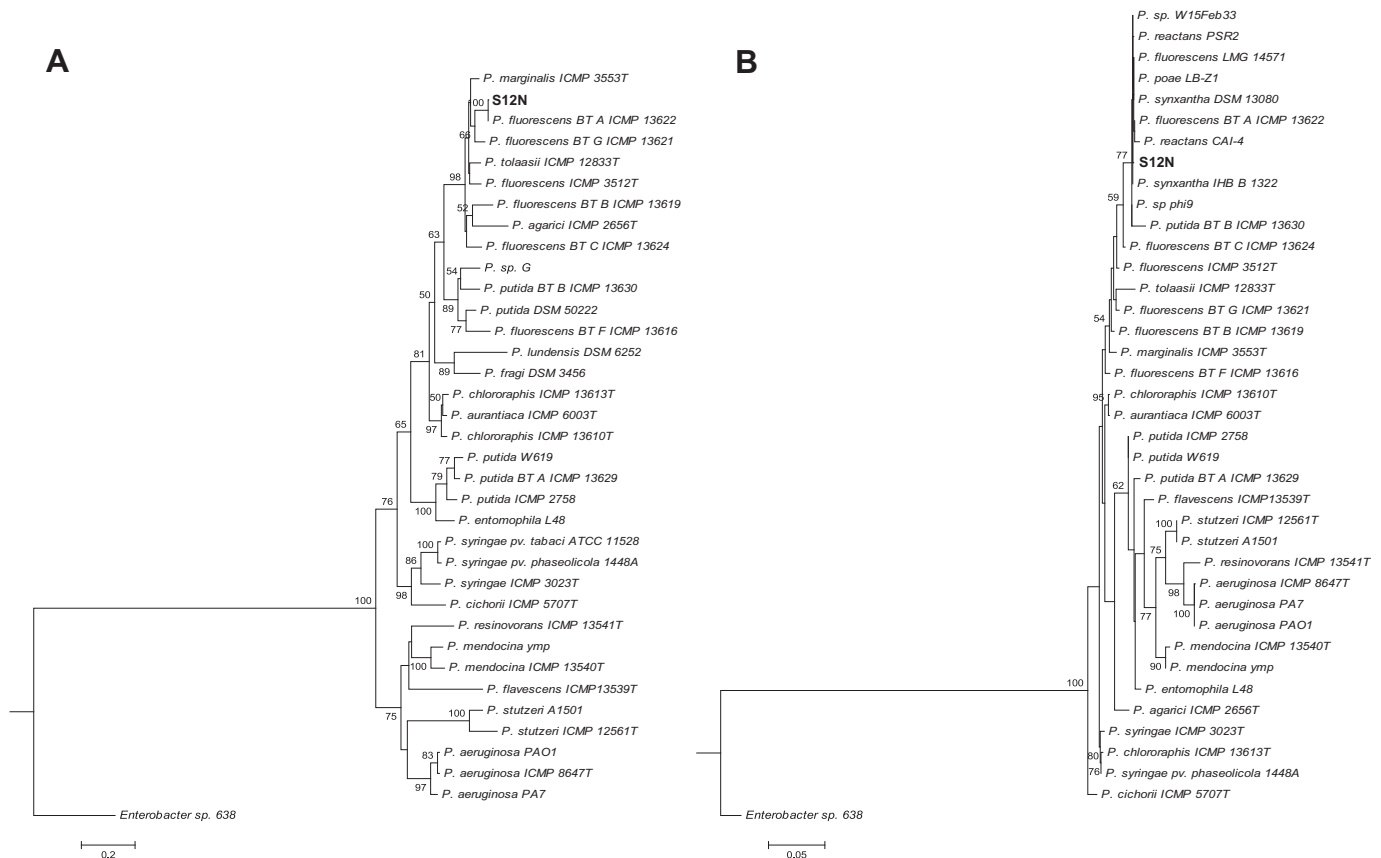
Fig. 2. Maximum likelihood phylogenetic trees of Pseudomonas fluorescens S12N isolated from black spots in dry-cured Iberian ham and Pseudomonas strains using carA (A) and 16S rRNA (B) genes. Bootstrap percentages of 50% or more are indicated at the branch points. Enterobacter was included as an outgroup. Strain and accession numbers are shown in Table 1.
