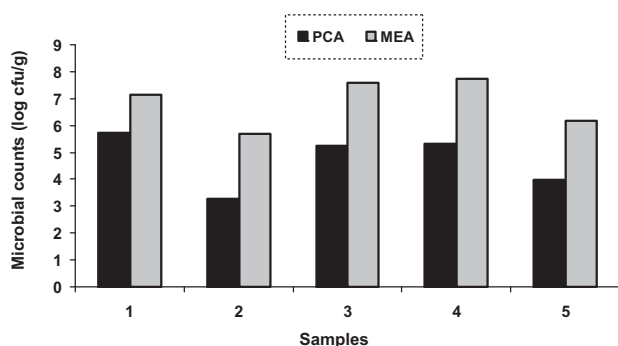
Fig. 1. Microbial population enumerated on Plate Count Agar (PCA) and Malt Extract Agar (MEA) of 5 dry-cured Iberian ham samples with black spot spoilage.
