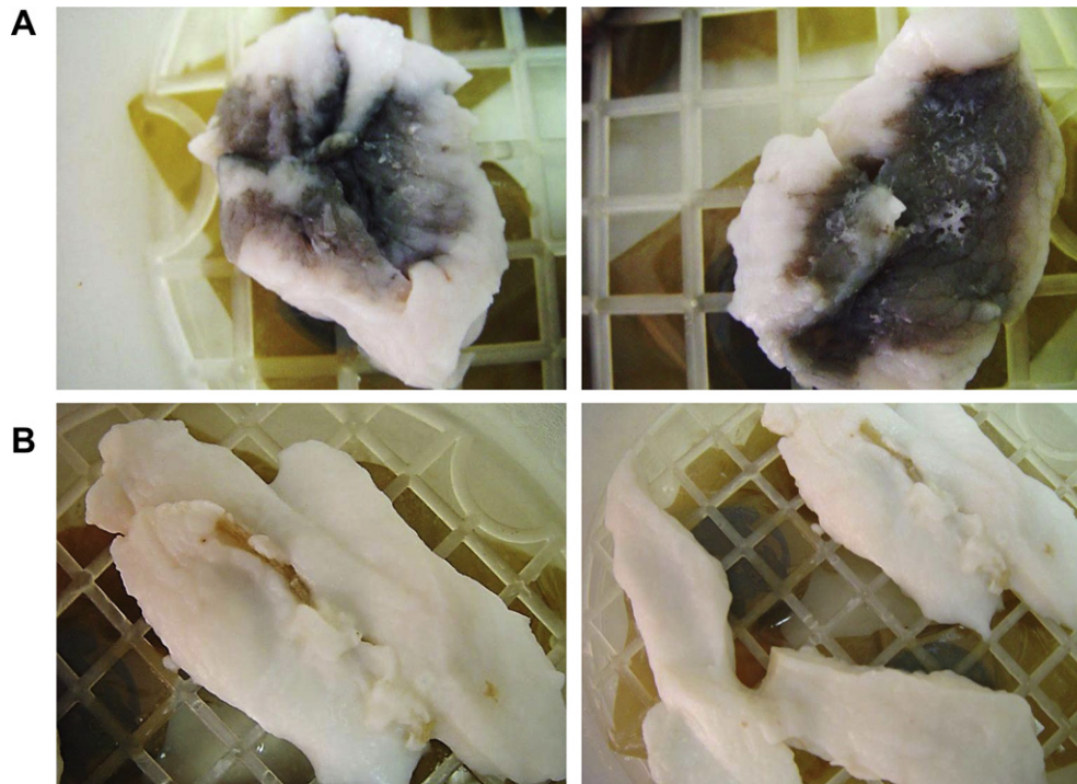
Fig. 4. Examples of black spot spoilage formation in fat tissues from non salted Iberian ham artificially contaminated with Pseudomonas fluorescens S12N after 15 days of incubation period at 10 °C (A). Alteration was not detected in either salted at 2% NaCl or non inoculated fat samples after 15 days of incubation at 10 °C (B).
